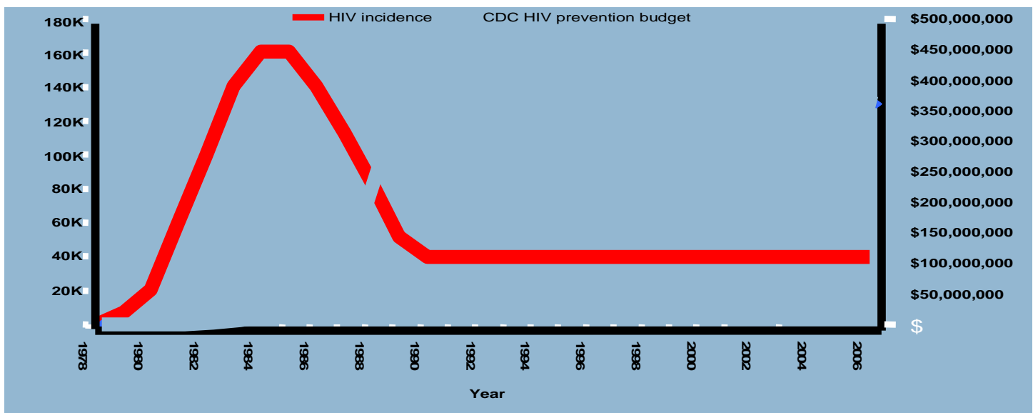
Estimated Annual HIV Incidence and CDC's HIV Prevention Budget (In 1993 Dollars), 1978-2006
